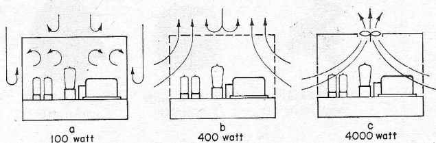
Fig. 1. Convection methoden
